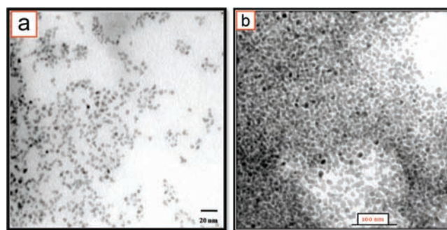
Figure 5. TEM images of (a) CdSe ripened in DMF for 8 h and (b) CdTe QDs ripened in DMF for 3 h.
