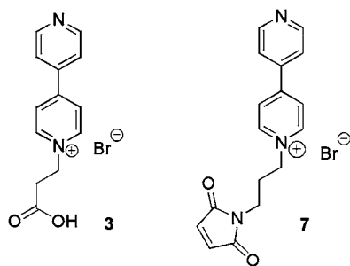
Figure 1. 4,4'-Bipyridinium salt-based twin ligands used to synthesize aqueous QDs.
